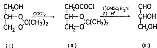
Scheme 1. Synthesis of DL-glyceraldehyde (III). DMSO = dimethyl sulfoxide
